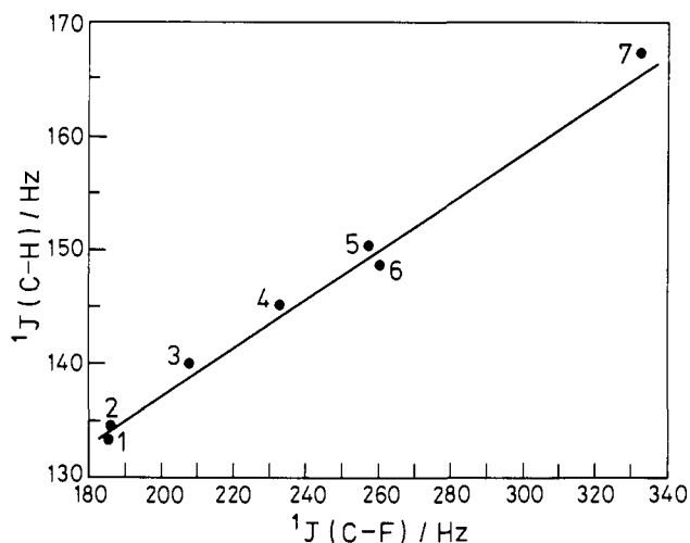
Figure 1. Plot of 1 J( 13 C-H) of the bridgehead carbon in the parent hydrocarbons vs. 1 J( 13 C-F) in the fluorides 1-7.
